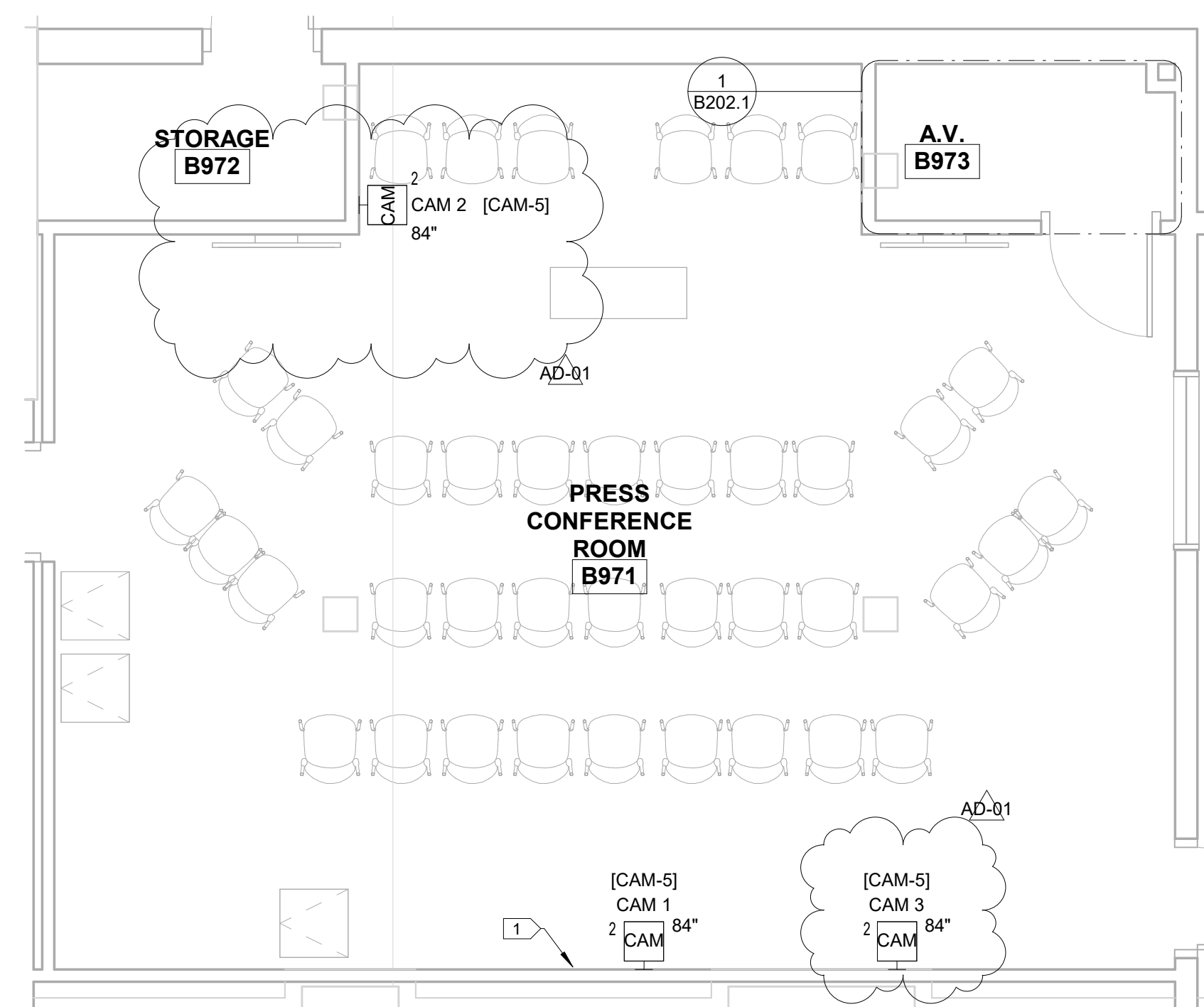
1 PRESS CONFERENCE ROOM-B971 ENLARGED FLOOR PLAN SCALE: 1/4" = 1'-0"
