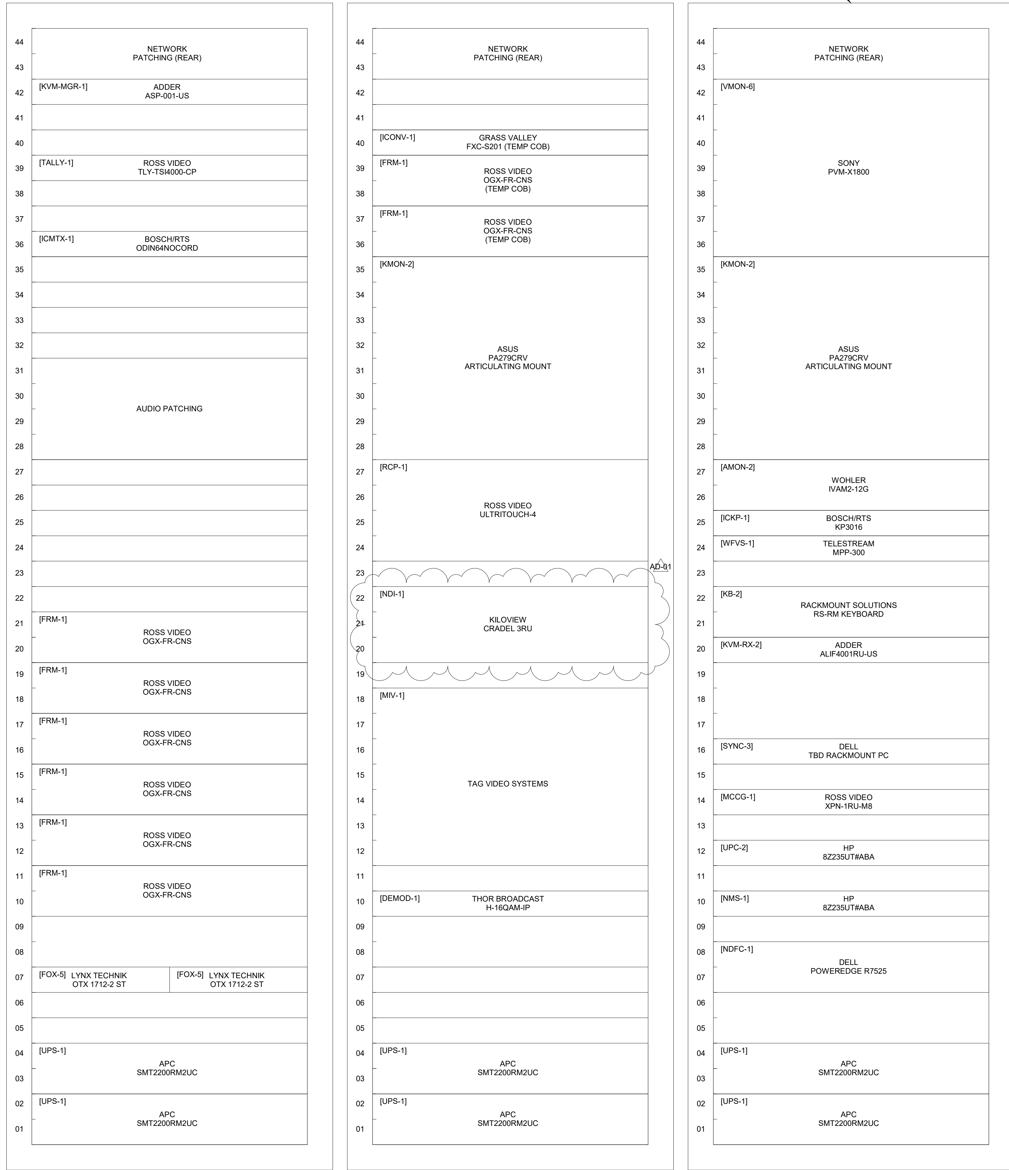
1 MEDIA HUB-B881 RACK ELEVATION 5-7
