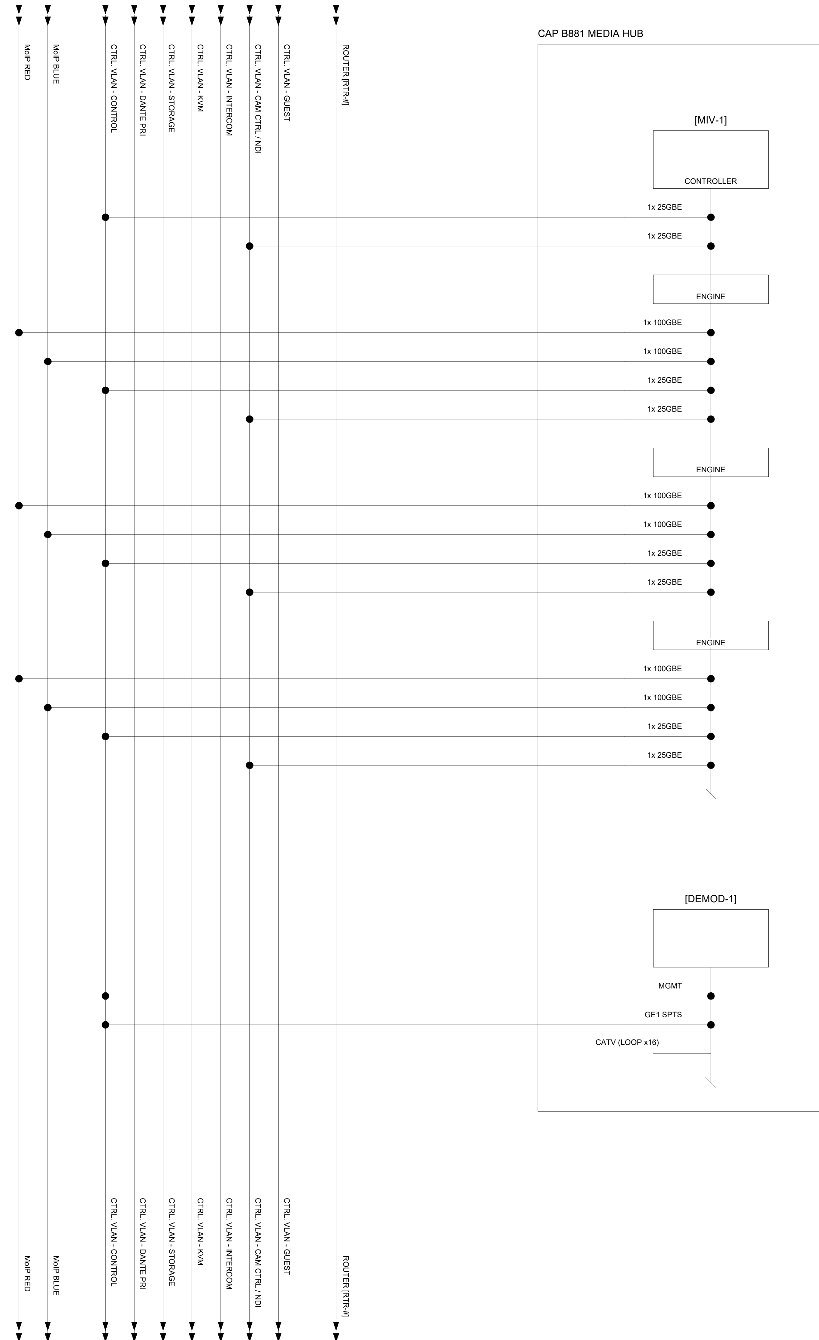
1 TRANSMISSION MULTIVIEW - FUNCTIONAL DRAWINGS
